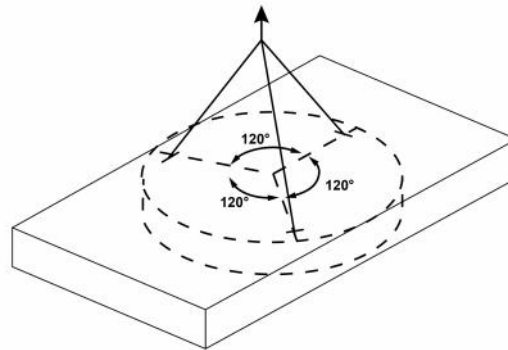
Three point lifting
